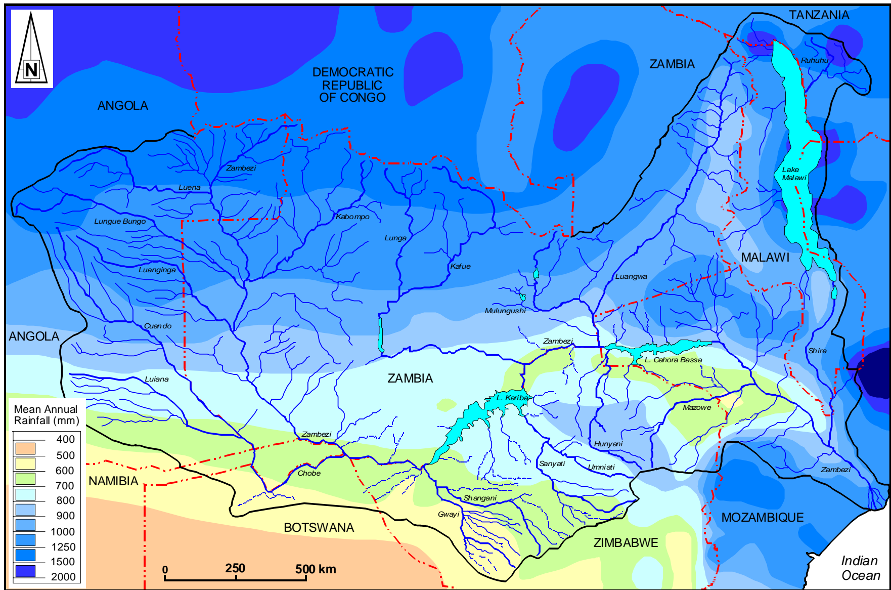
Figure 3.1: Sketch map showing the distribution of mean annual rainfall over the Zambezi basin, plus major rivers and lakes.
